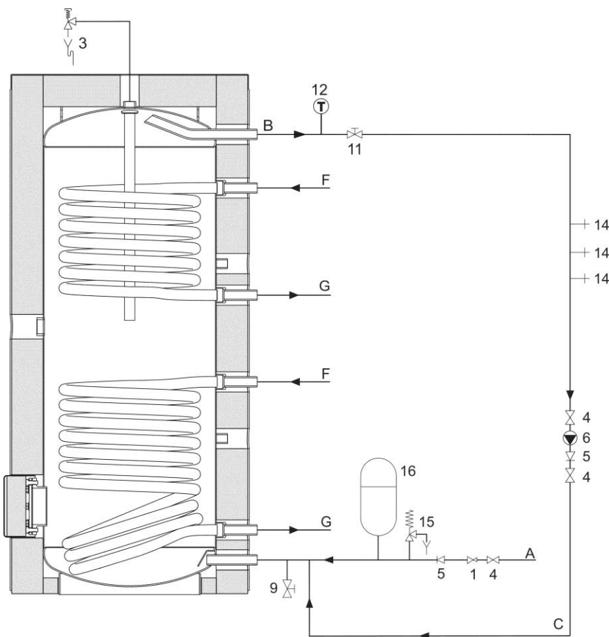
Installation Diagram
