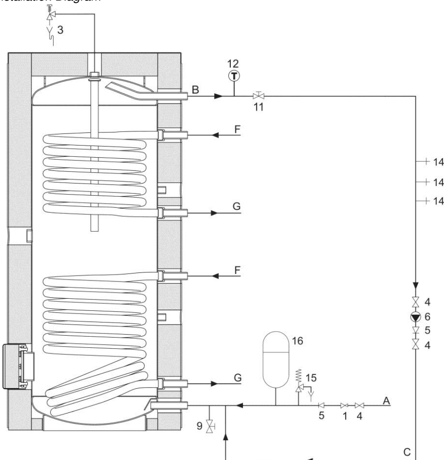
Installation Diagram
