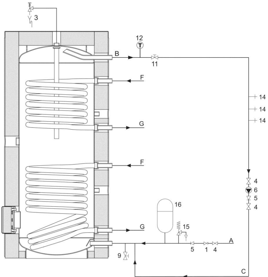
Installation Diagram
