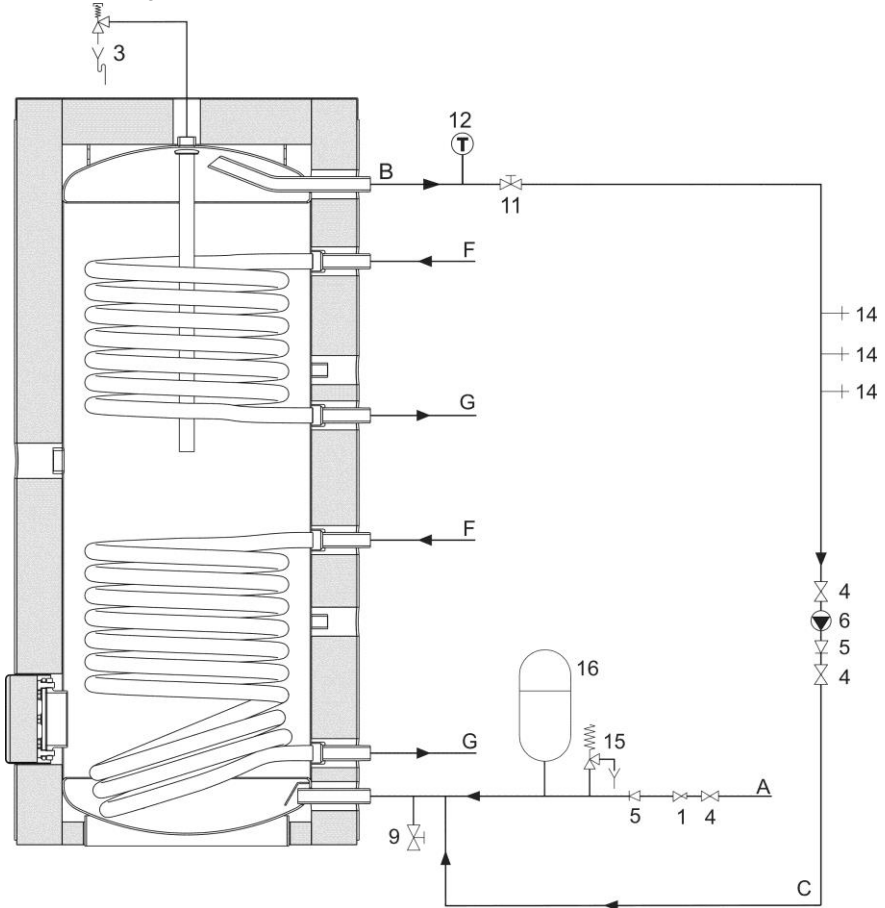
Installation Diagram
